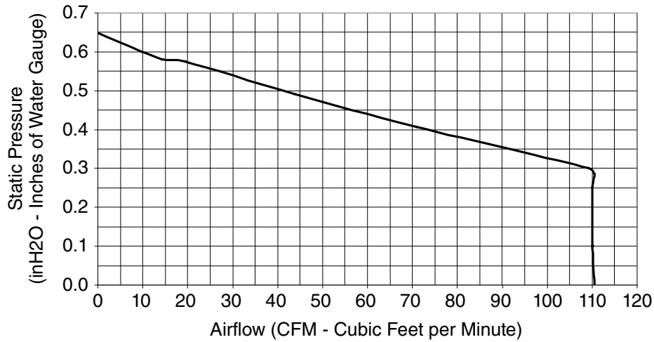
XB110 - 6" DUCT
