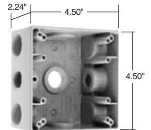
Dimensions for Two Gang Box
