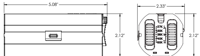
2 1/2" CEILING CUTOUT
