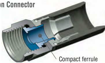
Compact ferrule
