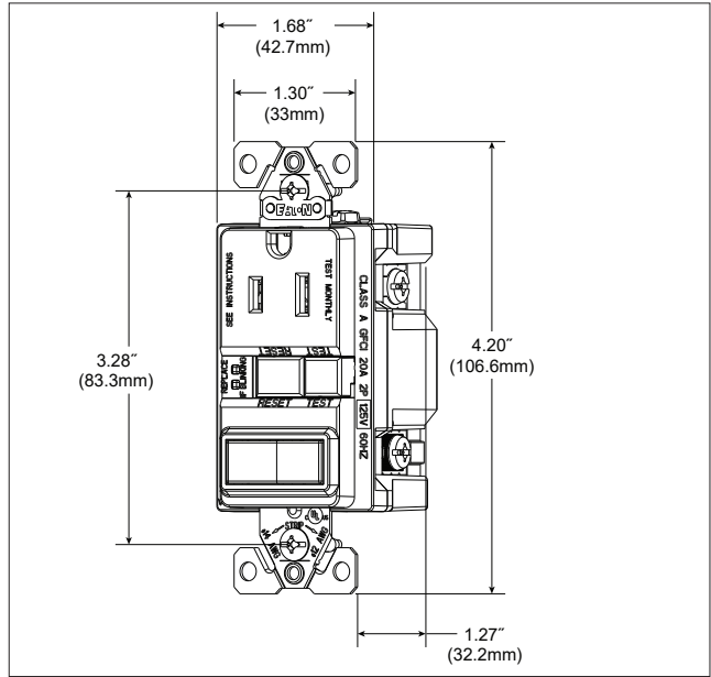
Figure 1. TRSGFS15 dimensions
