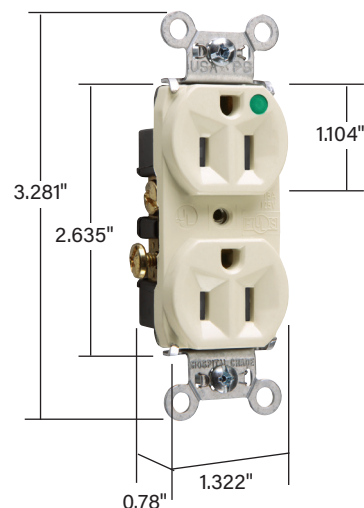
Dimensions for 15 & 20 Amp TR8200HLA
