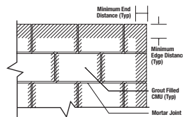
Wall Face Permissible Anchor Locations (Un-hatched Area)
