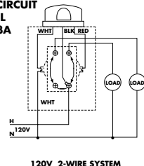
120V 2-WIRE SYSTEM
