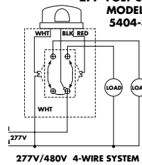
277V/480V 4-WIRE SYSTEM
