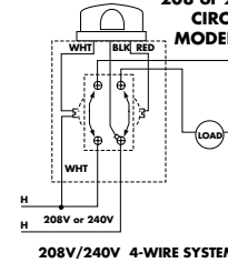
208V/240V 4-WIRE SYSTEM
