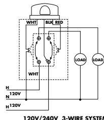
120V/240V 3-WIRE SYSTEM
