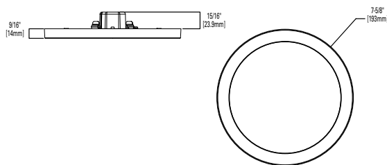
SMD6RXXXWH
