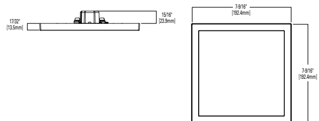
SMD6SXXXWH
