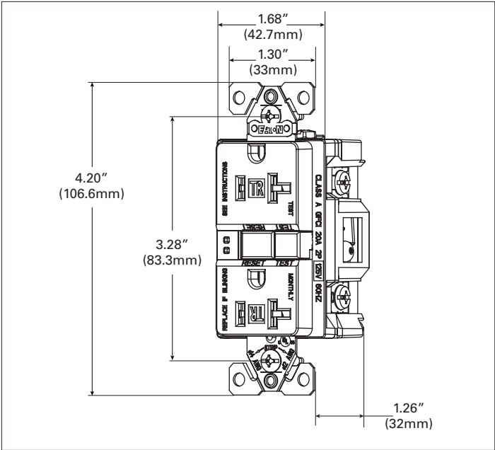
Figure 6. TRSGF20 & TRSGF20F Line art with dimensions
