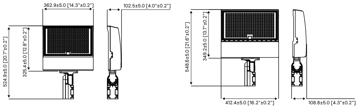
205W Slipfitter Slim Flood 120-150-205W/3CCT/UN3/SF
