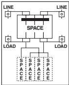
Fig. F U281E1 Series/Parallel
