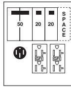
Fig. G U076C010 BR54U, (2) 5-20R2GFCI
