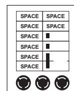
Fig. E U239G L6-30R, (2) L5-20R
