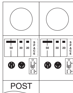
Fig. C M075CB6010, R075CB6010, R075CB6010FMG BR54U, R32U, 5-20R2GFCI
