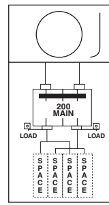
Fig. E R281C1034 Series
