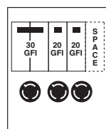
Fig. D U870G6 L6-30R, (2) L5-20R
