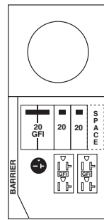
Fig. G M038CB1033 6-20R, (2) 5-20R2GFCI
