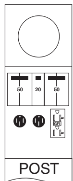
Fig. A M004CP6010 (2) BR54U, 5-20R2GFCI
