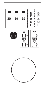
Fig. F R031C010U R32U, (2) 5-20R2GFCI
