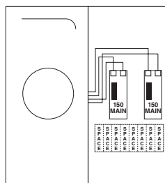
Fig. C RS43308C, RS43308CGP THQD22150WL
