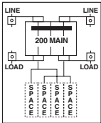
Fig. E U281C1 Series/Parallel
