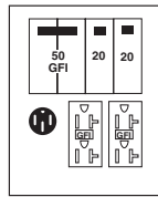
Fig. H U076C033 BR54U, (2) 5-20R2GFCI
