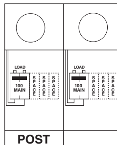
Fig. G M101CB6HP, R101CB6HP Series
