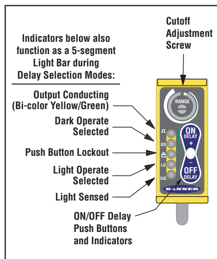
Figure 1. Q60LAF features
