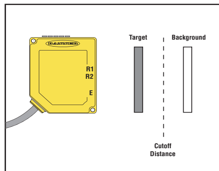
Figure 5. Set cutoff distance approximately midway between the farthest target and the closest background
