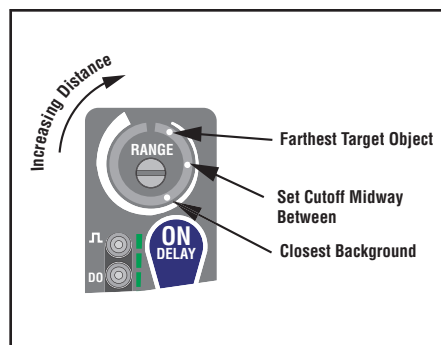
Figure 6. Setting the cutoff distance
