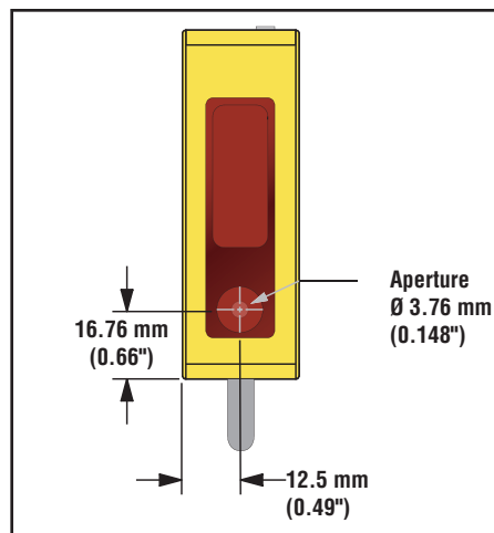
Figure 10. Laser aperture location
