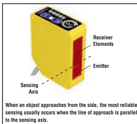
Figure 3. Q60 sensing axis
