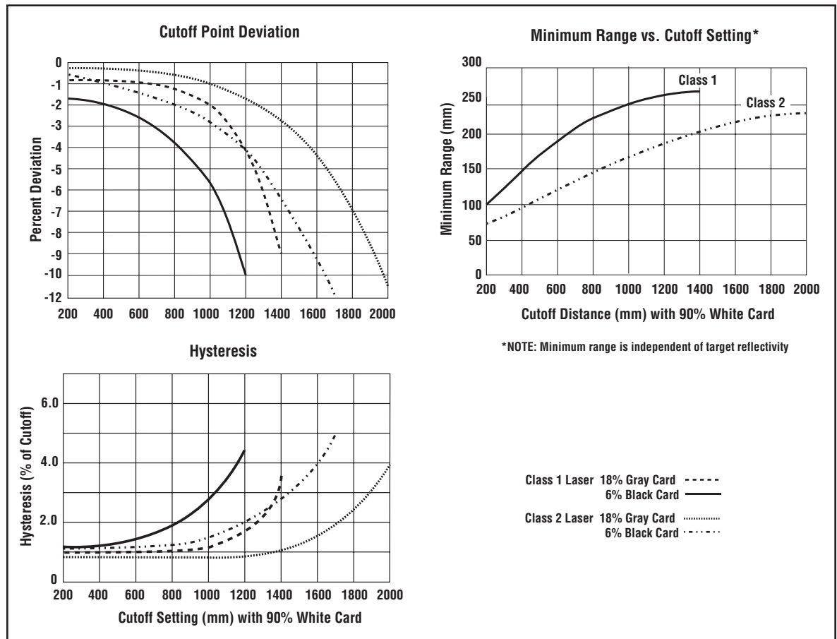
Figure 4. Q60LAF performance
