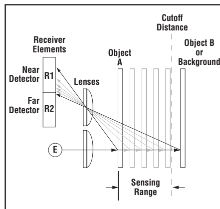
Figure 2. Adjustable field sensing concept
