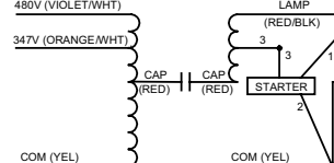
Wiring Diagram 23
