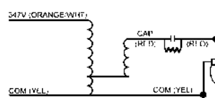
Wiring Diagram 6
