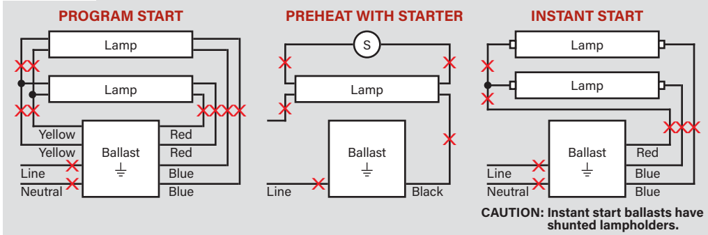
FIGURE A Typical Ballast Wiring Configurations
