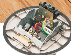
Brass Trapdoor style FLBT6615MB (open and back)
