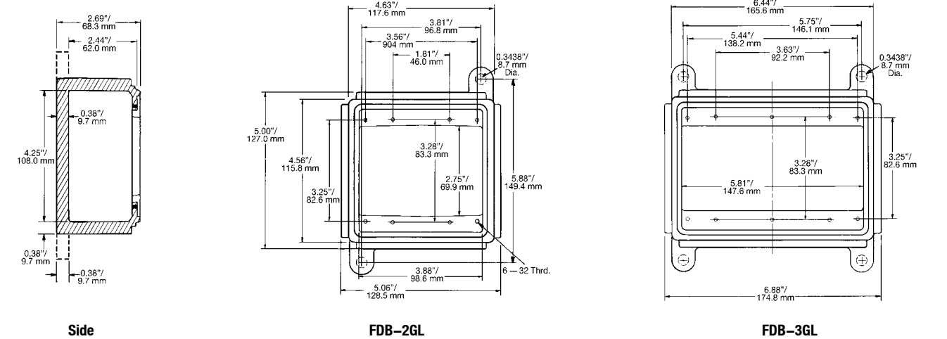
FDB Two and Three Gang Single Cover Boxes.
