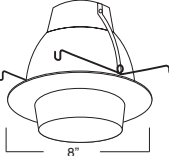
B663PB PAR30 GIMBAL RING
