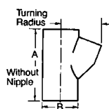
EYSF 1/2" — 3" EYSM 1/2" — 1"
