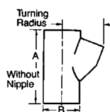
EYSF 1/2" — 3" EYSM 1/2" — 1"
