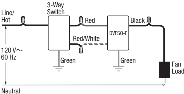
DVFSQ-F - Load-Side
