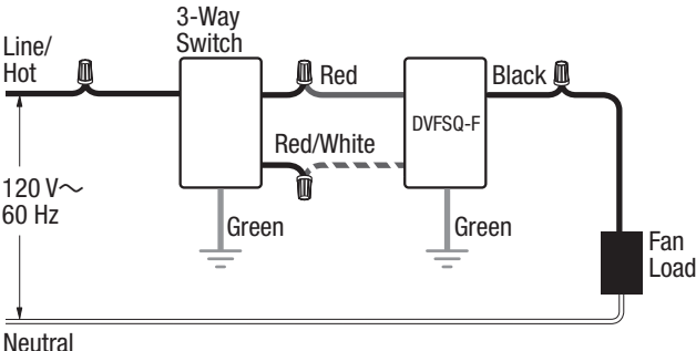
DVFSQ-F - Load-Side
