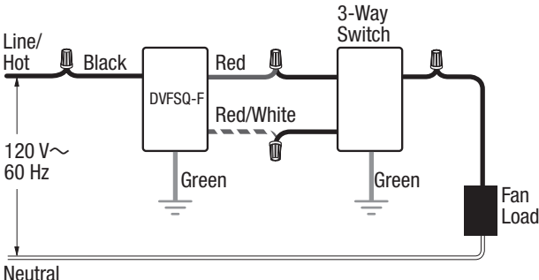
DVFSQ-F - Line-Side
