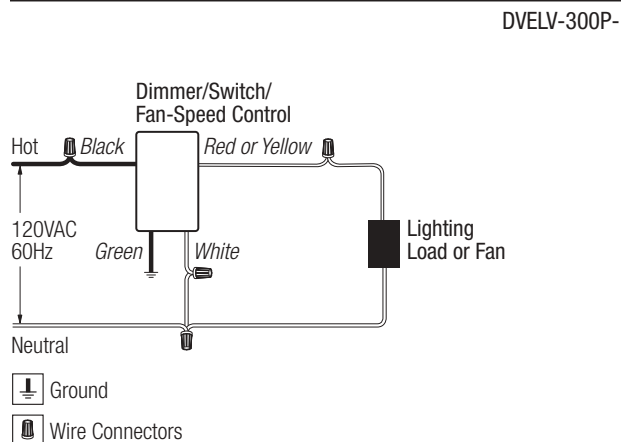
Wiring Diagram 3 Single-Pole Wiring
