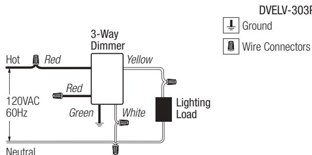
Wiring Diagram 5 3-Way Used as Single Pole
