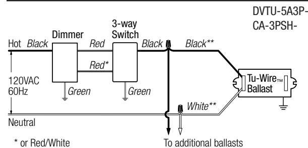
Wiring Diagram 11 3-Way Wiring
