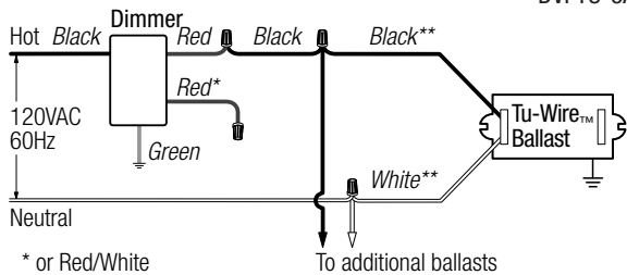
Wiring Diagram 10 Single-Pole Wiring
