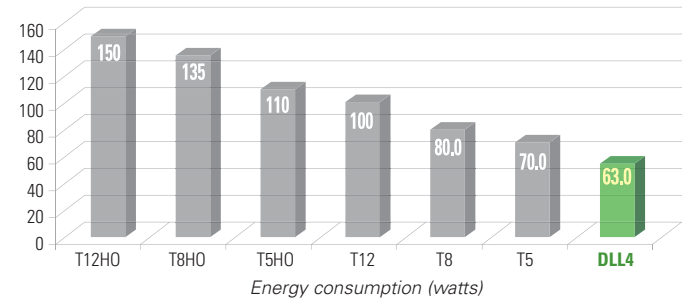
4 foot DLL linear LED vs. fluorescent
