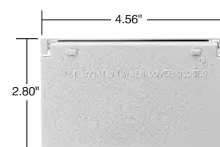
Dimensions for One Gang Horizontal 1 Self-Closing Lid
