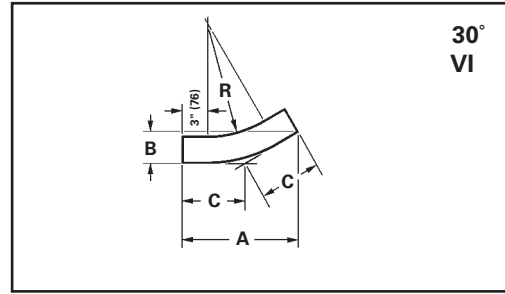
30° Vertical Inside
