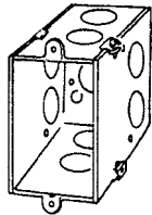
3-1/2" Deep, Gangable; Two nail holes each side
