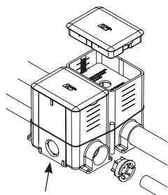
1 1/4" trade size knockout opening (both sides)
