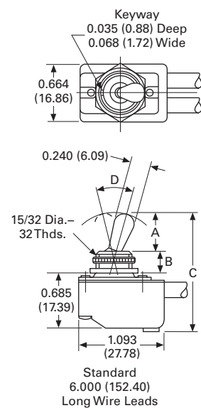
8391K107 and K108 1PST Maintained (Wire Lead)
