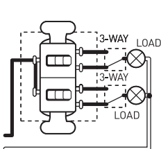
COMMON FEED
