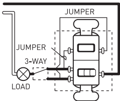
WIRED AS NIGHT LIGHT (Breakoff Tab Removed)
