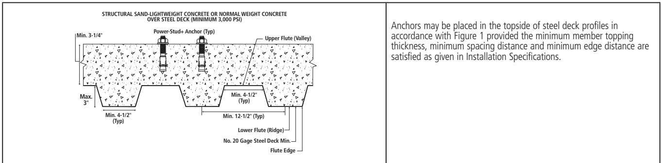
Figure 2A - Power-Stud+ SD1 Installation Detail for Anchors in the Topside Of Concrete Over Steel Deck Floor and Roof Assemblies (See Dimensional Profile Requirements)
