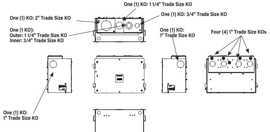
EFB45S Knockout Locations & Sizes
