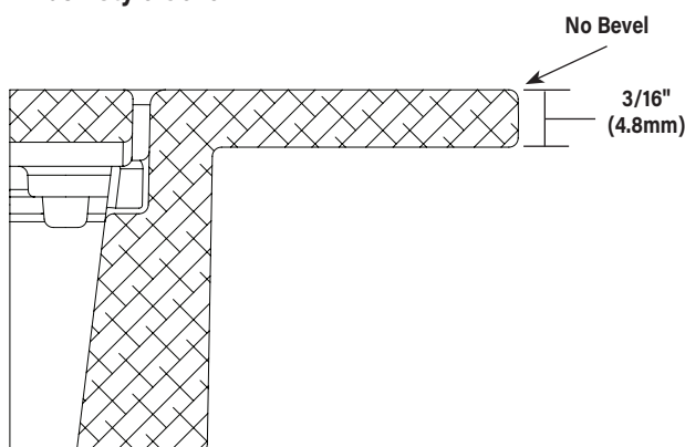
Flush Style Cover
