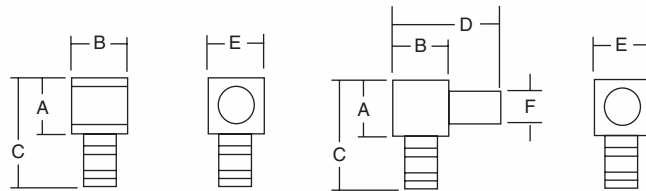
Female Disconnect
