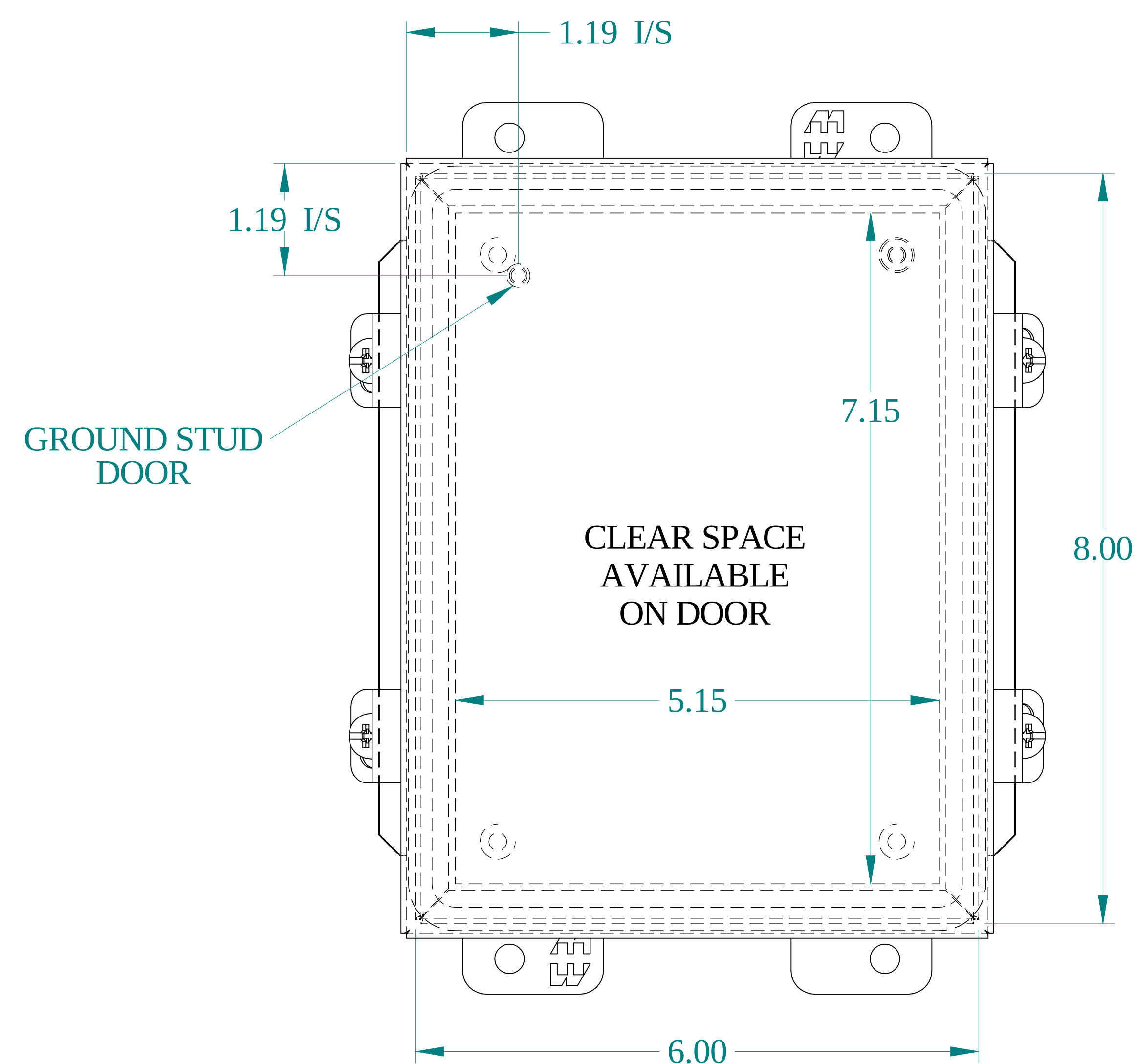
FRONT VIEW
