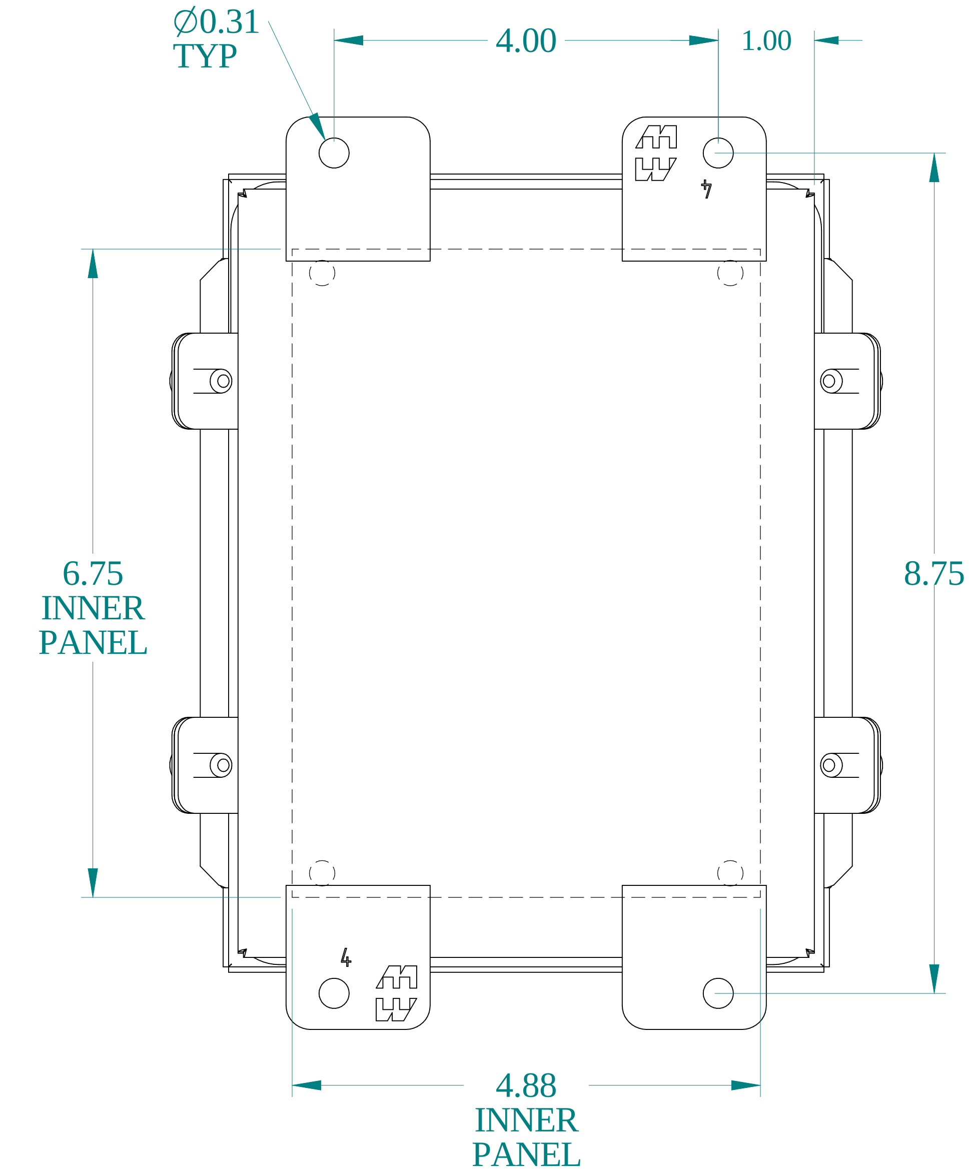
BACK VIEW
