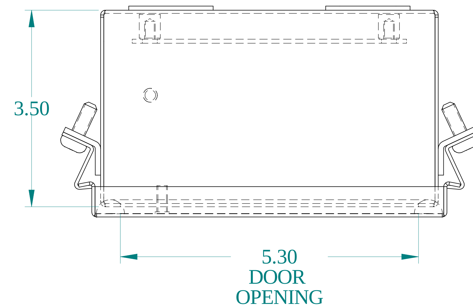
TOP VIEW
