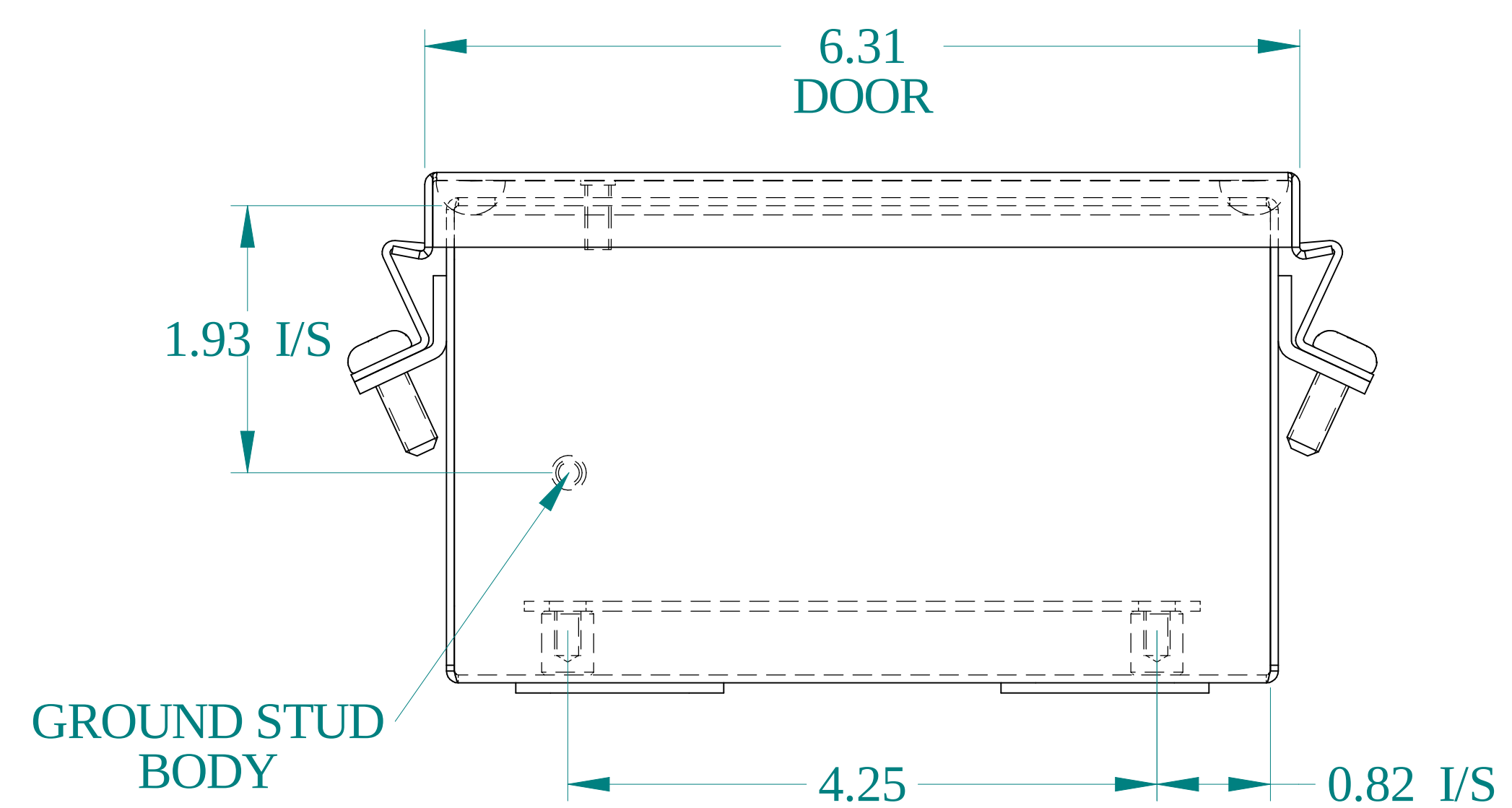
BOTTOM VIEW
