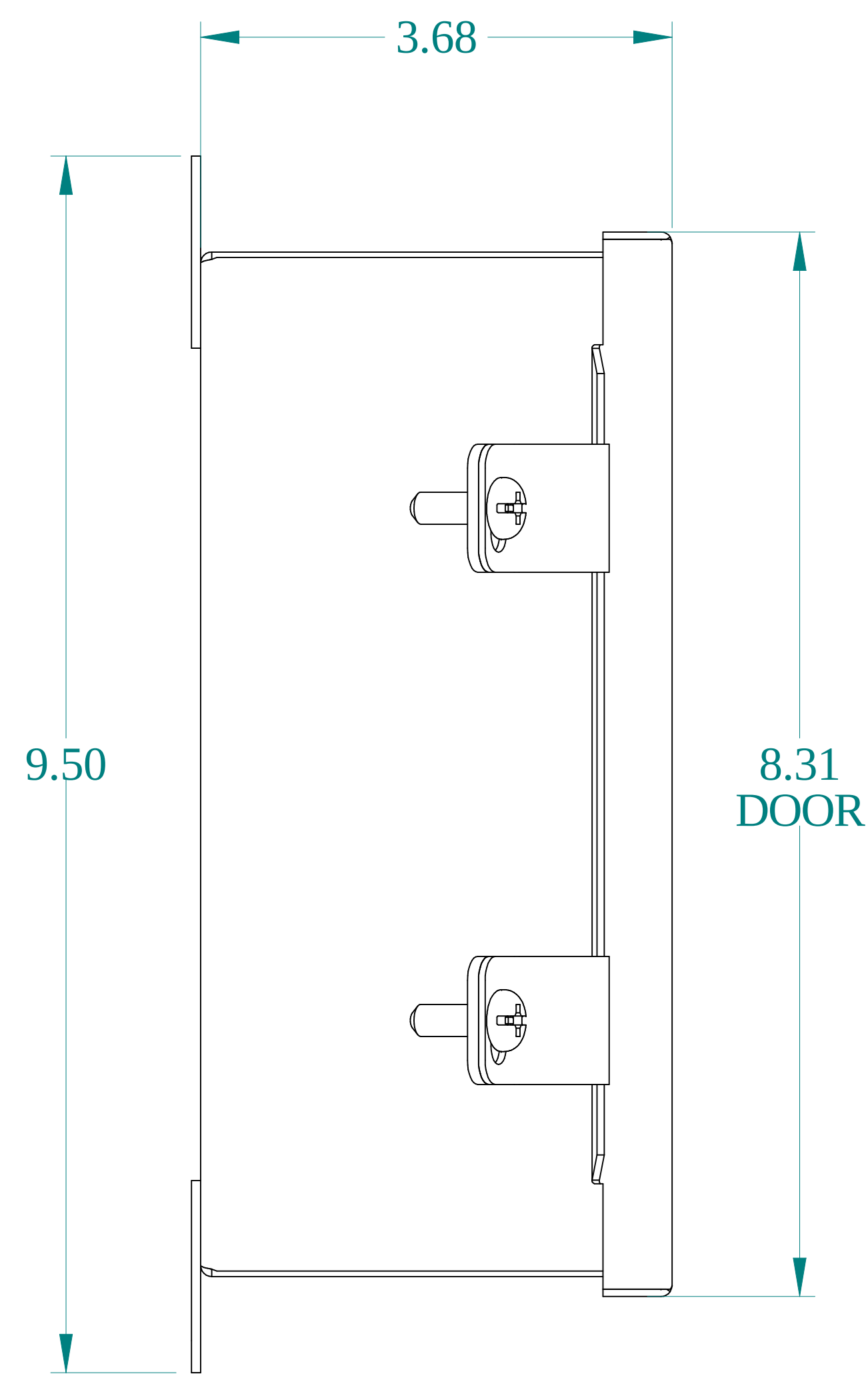
SIDE VIEW
