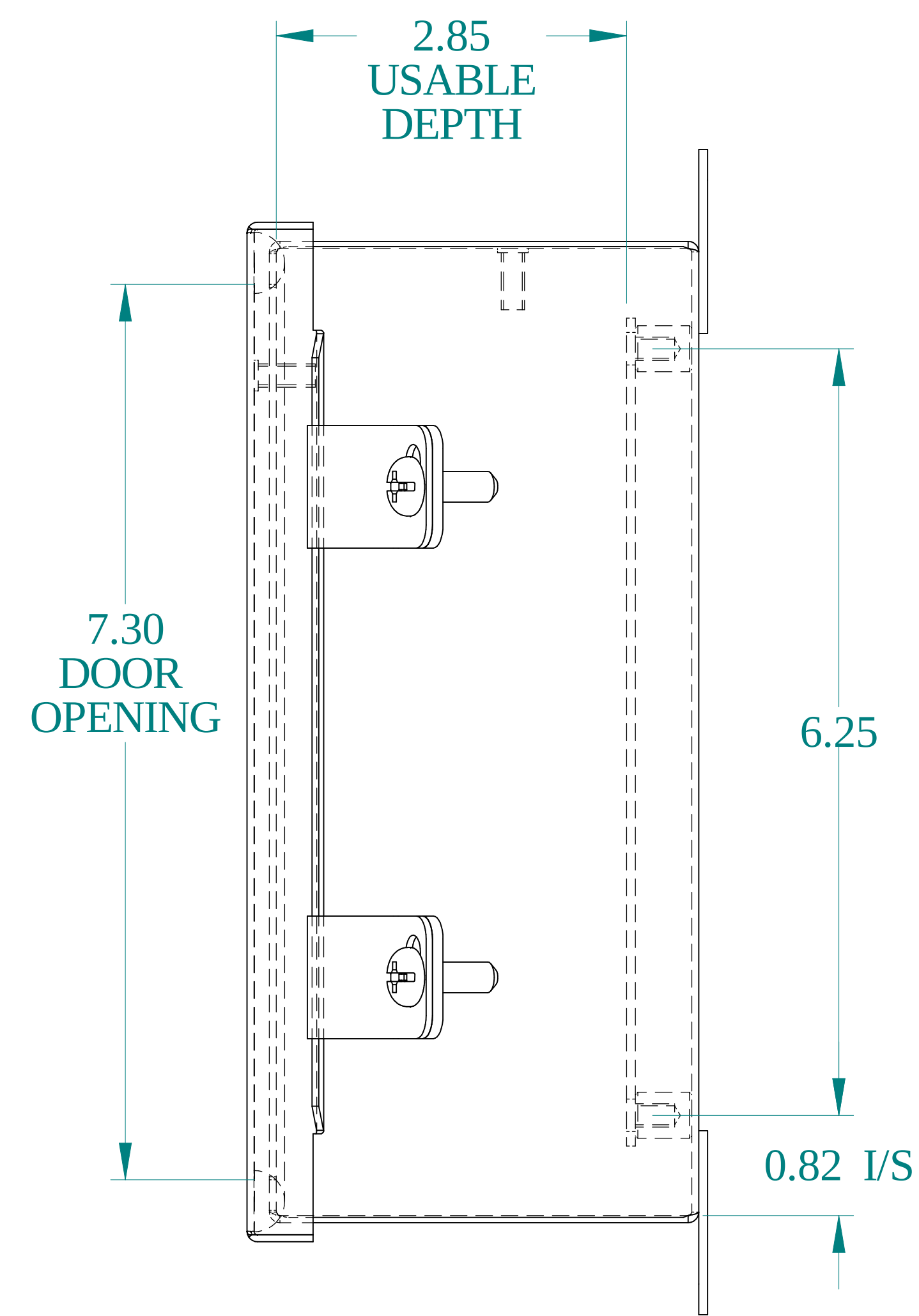
SIDE VIEW
