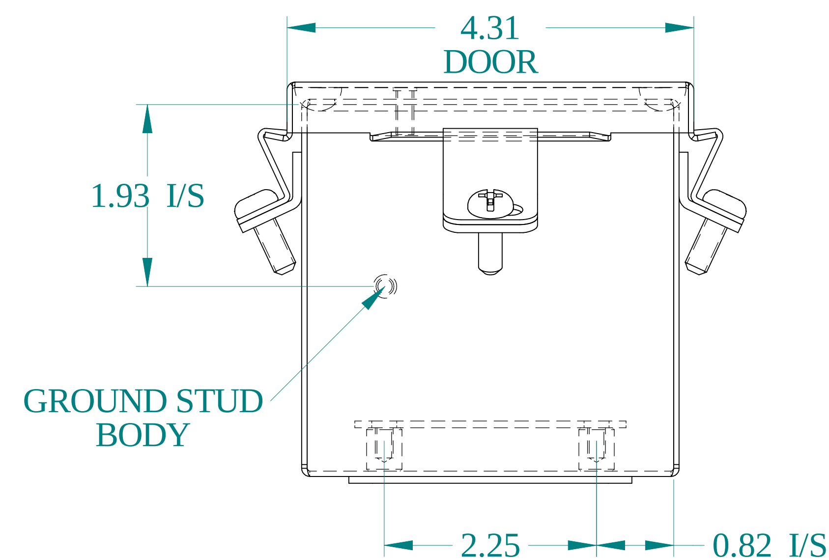
BOTTOM VIEW
