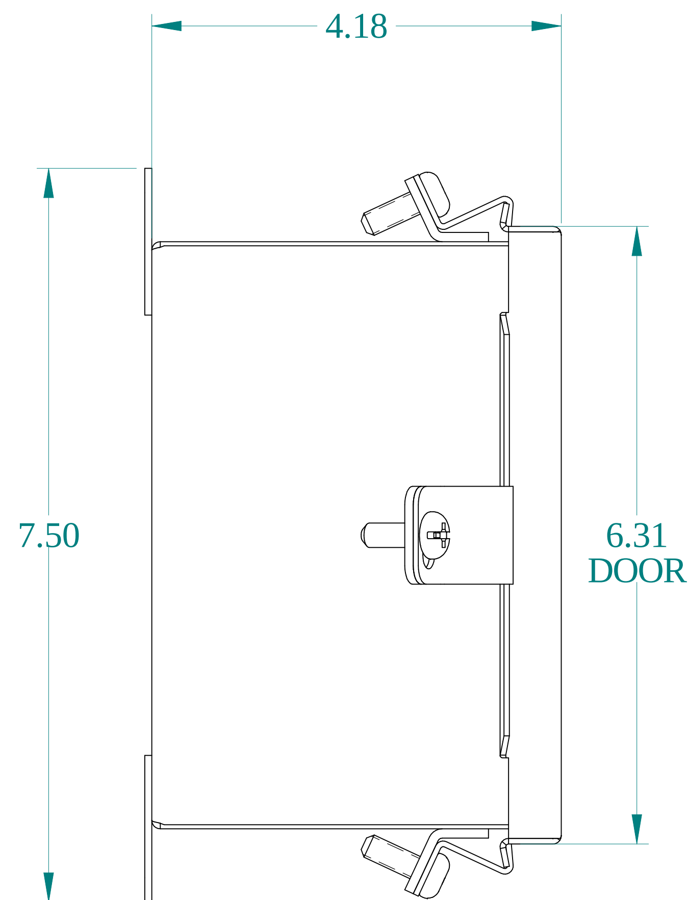
SIDE VIEW
