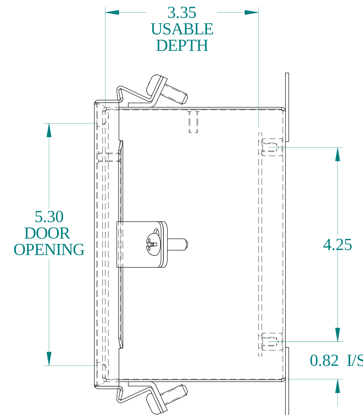
SIDE VIEW
