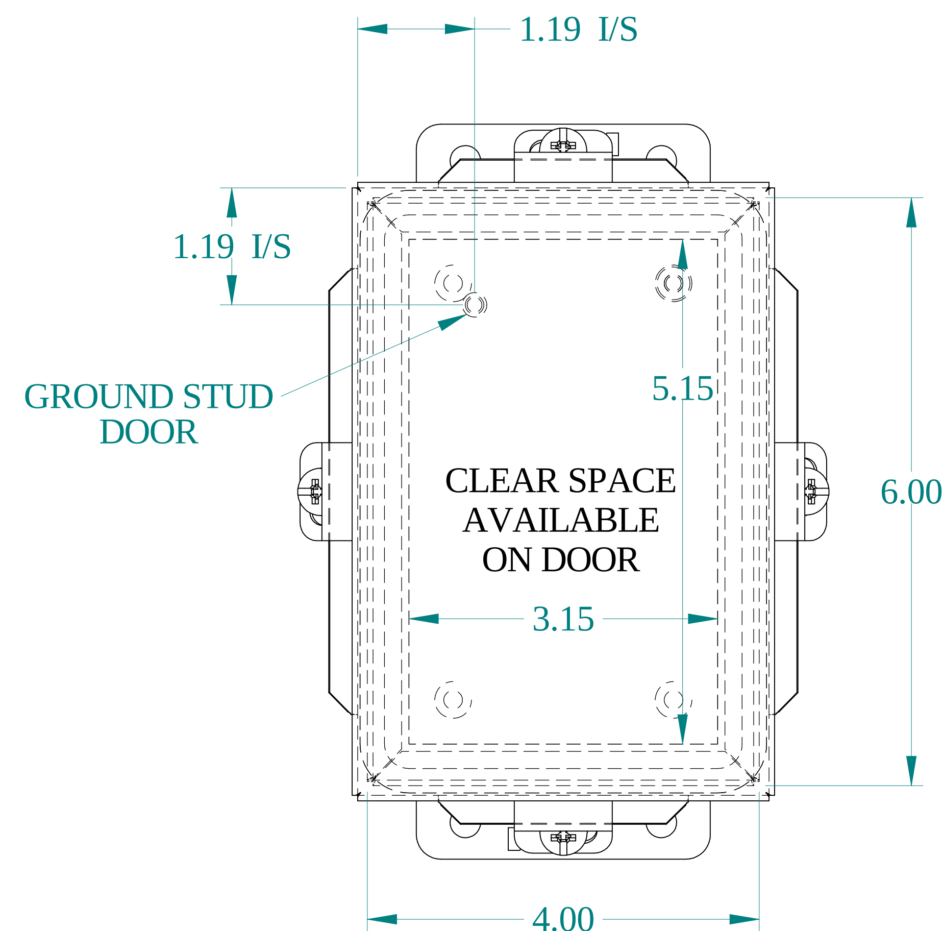
FRONT VIEW
